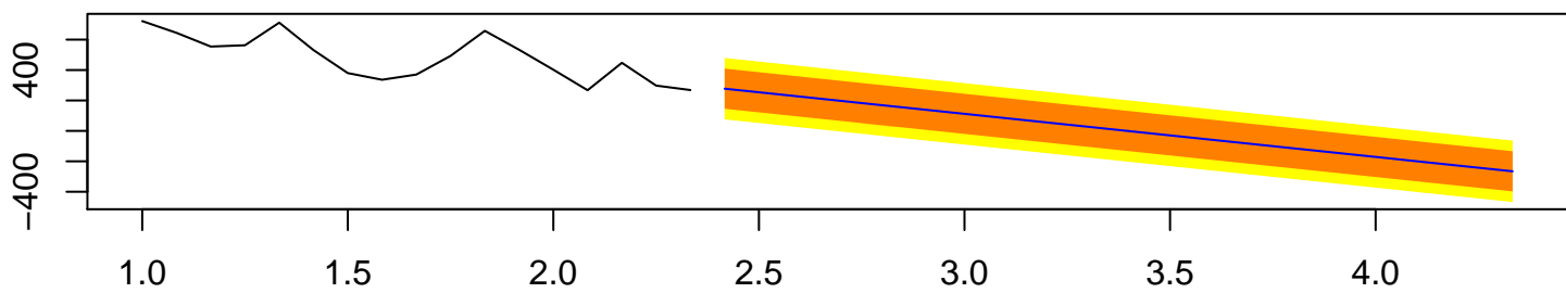
Forecasts from ETS(A,A,N)
