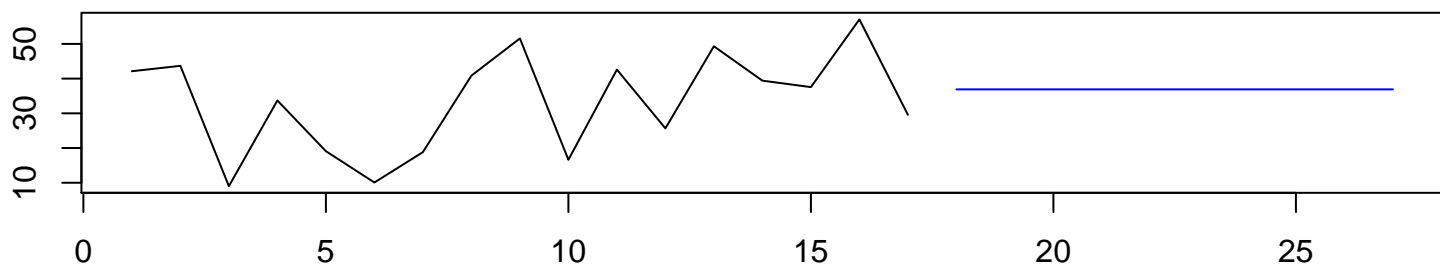
Forecasts from Croston's method
