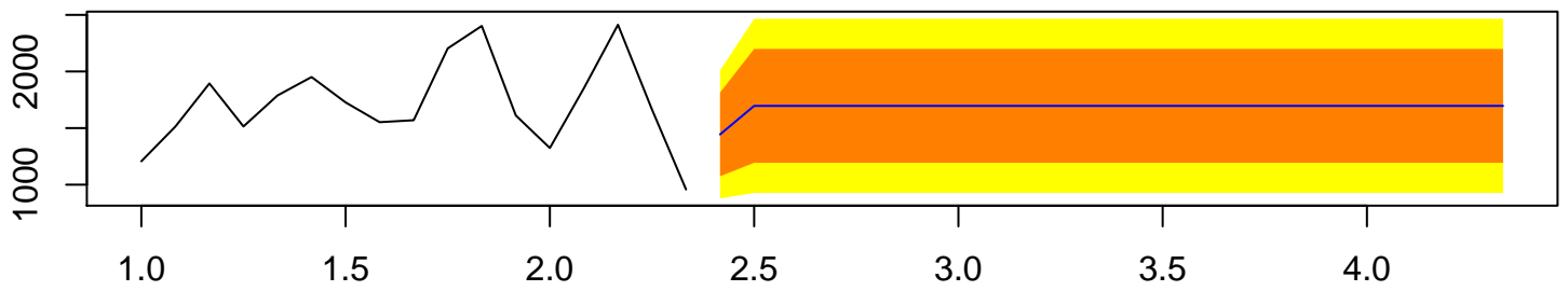
Forecasts from ARIMA(0,0,1) with non-zero mean
