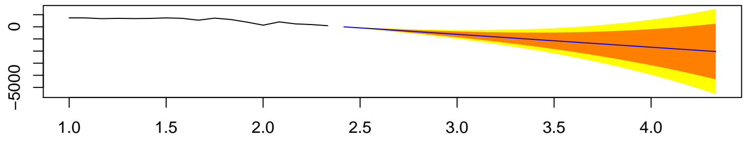
Forecasts from ETS(M,A,N)
