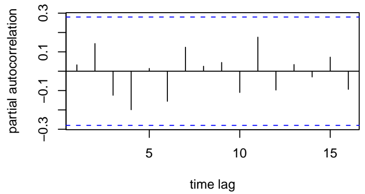
Residual PACF
