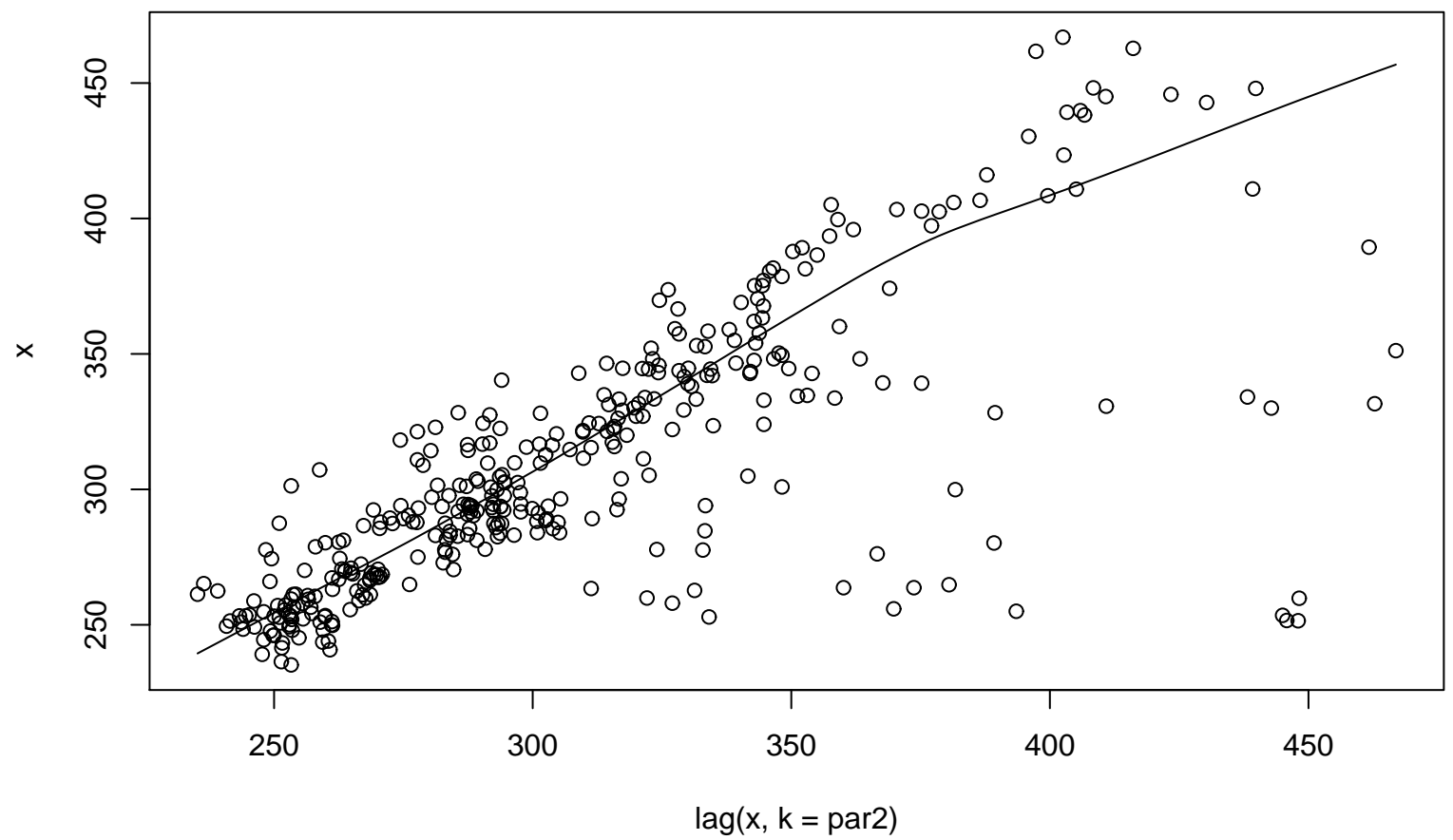
Lag plot (k=5), and lowess
