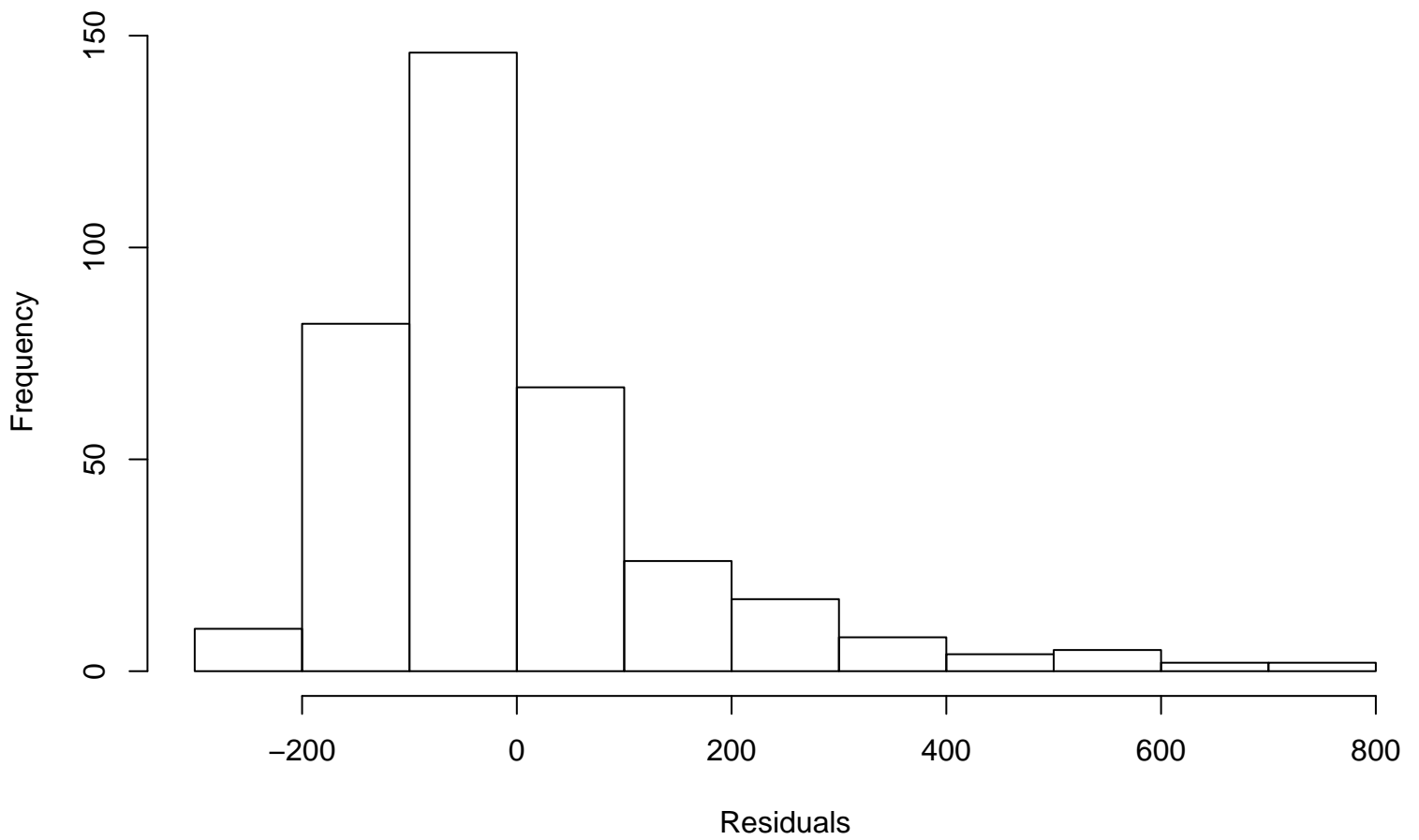
Residual Histogram
