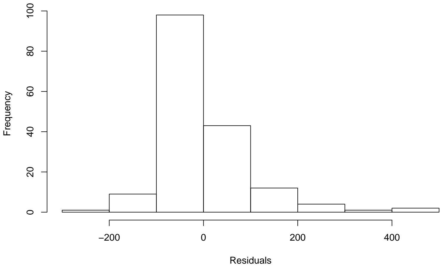
Residual Histogram
