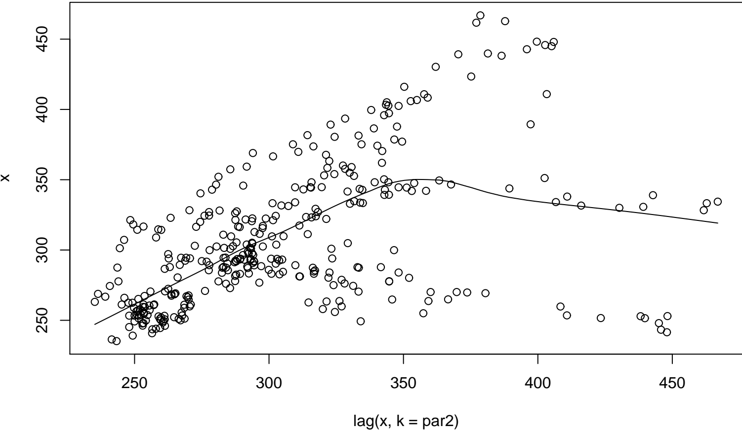
Lag plot (k=10), and lowess
