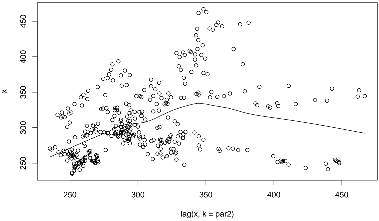
Lag plot (k=15), and lowess
