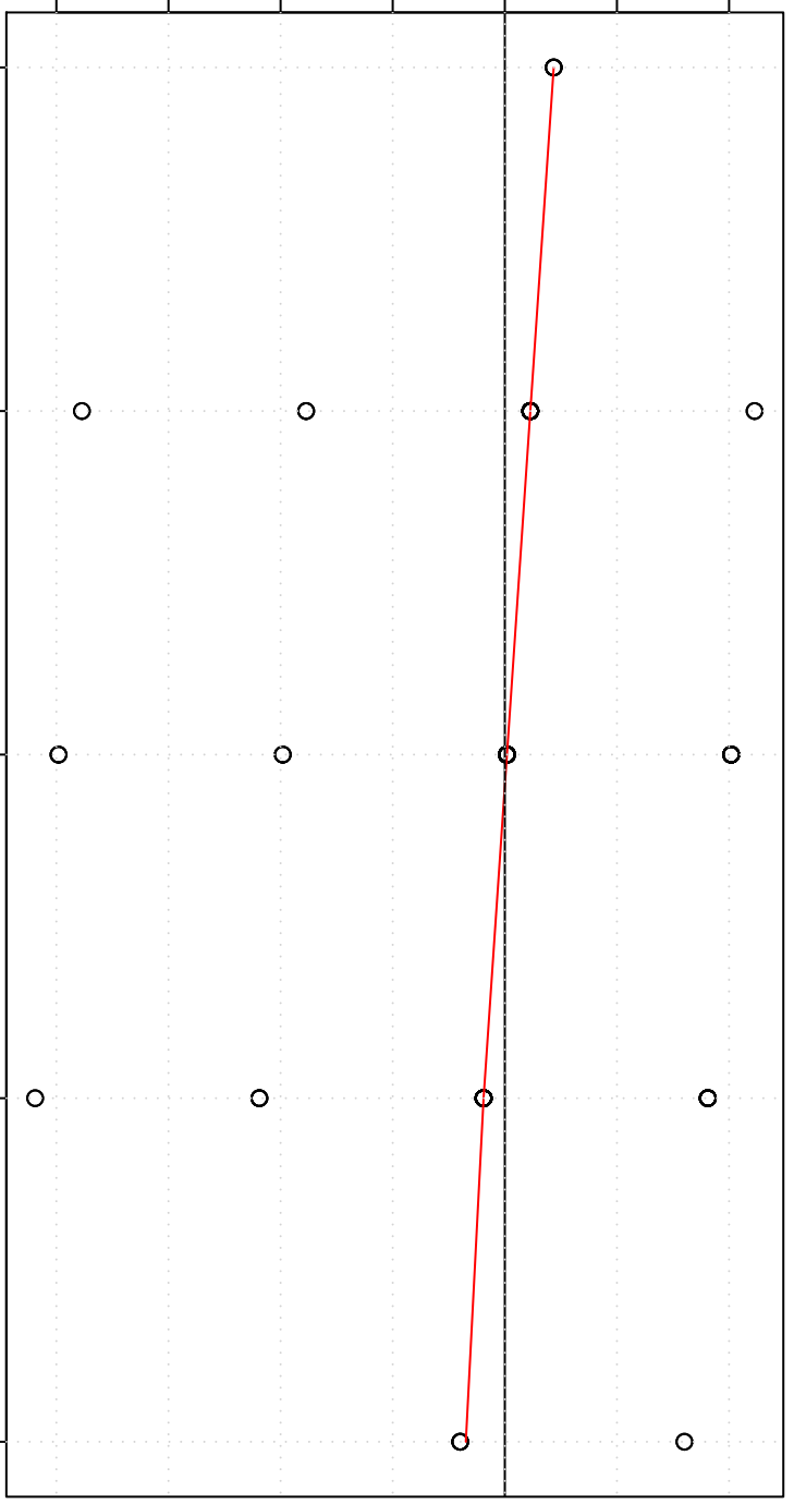
Scatterplot, lowess, and regression line
