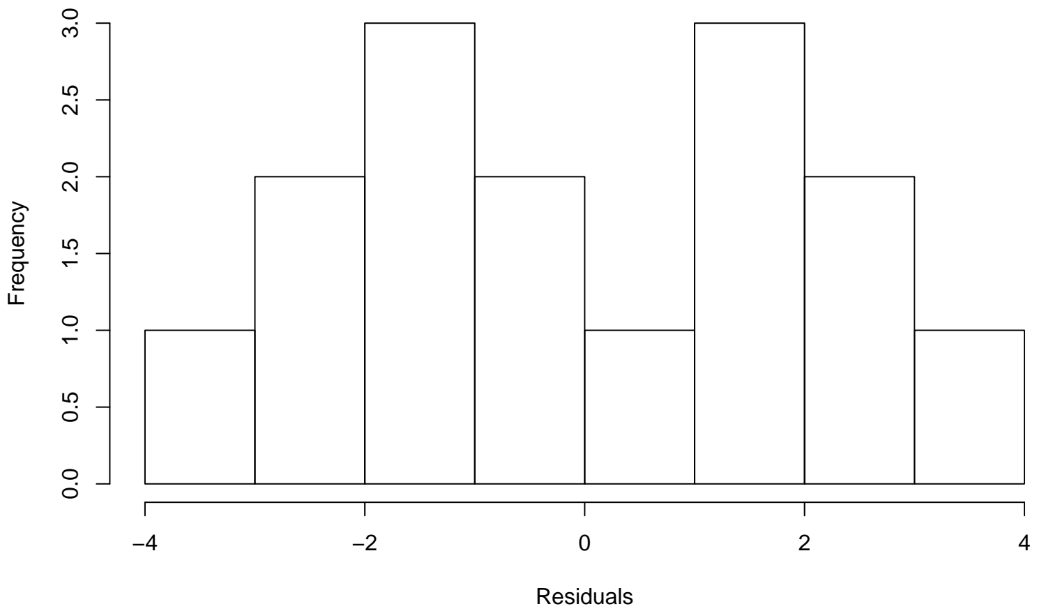
Residual Histogram
