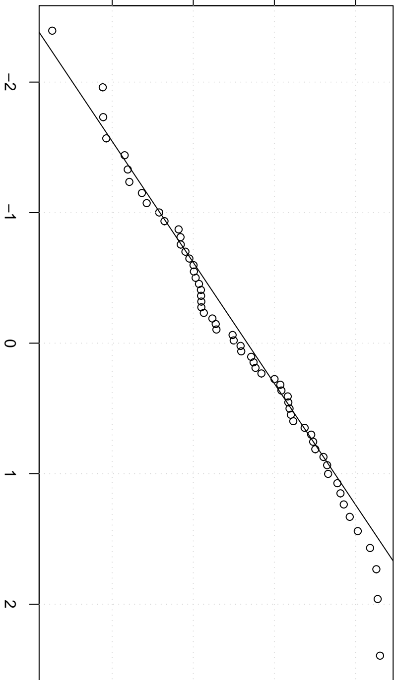
Normal Q-Q Plot
