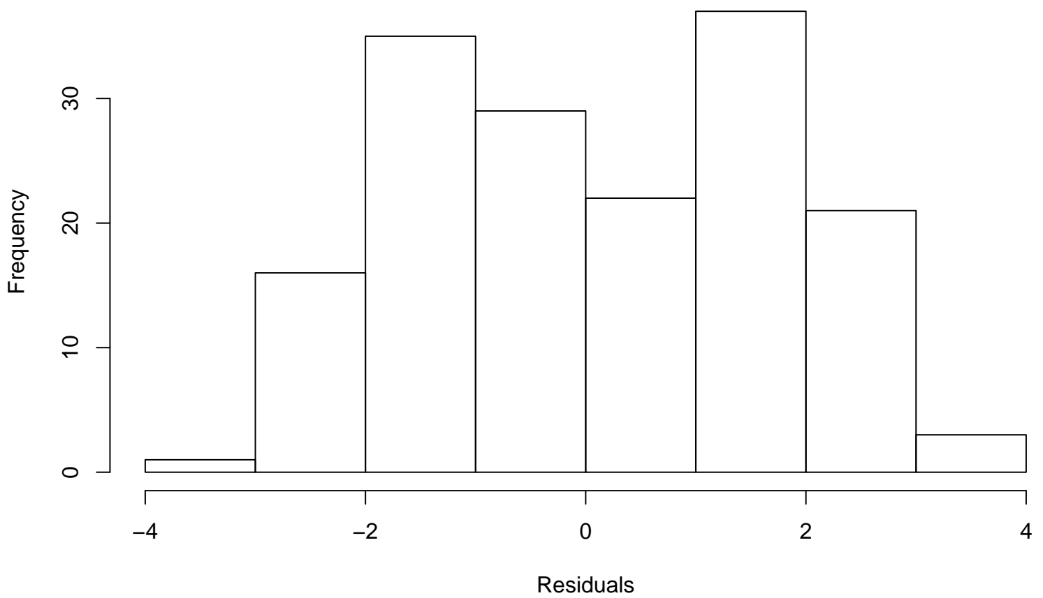
Residual Histogram
