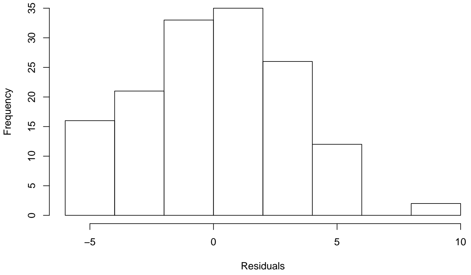
Residual Histogram
