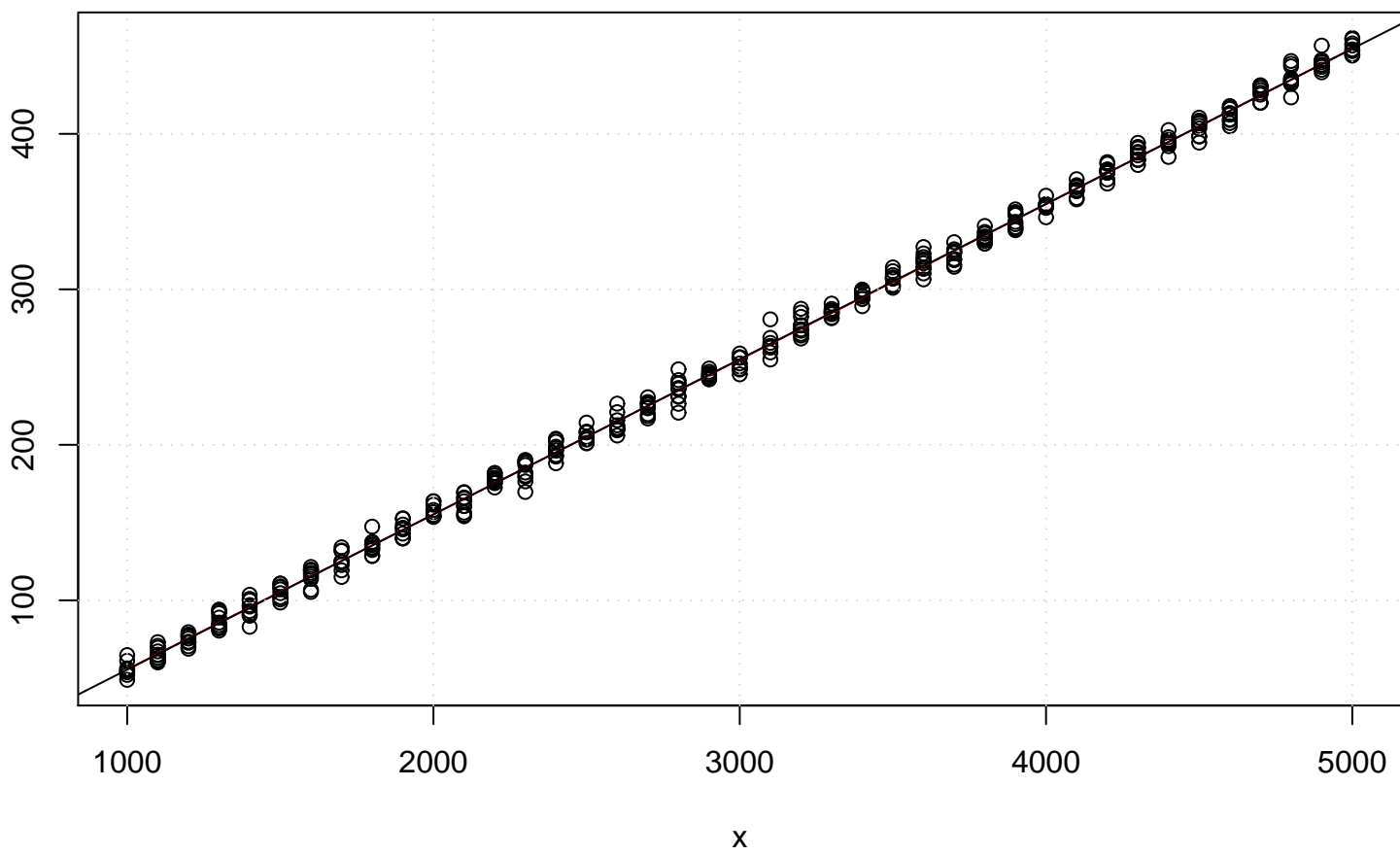
Scatterplot, lowess, and regression line
