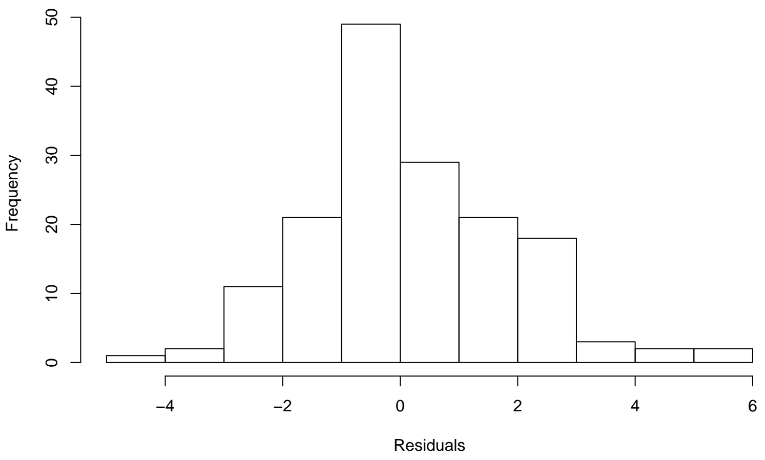
Residual Histogram
