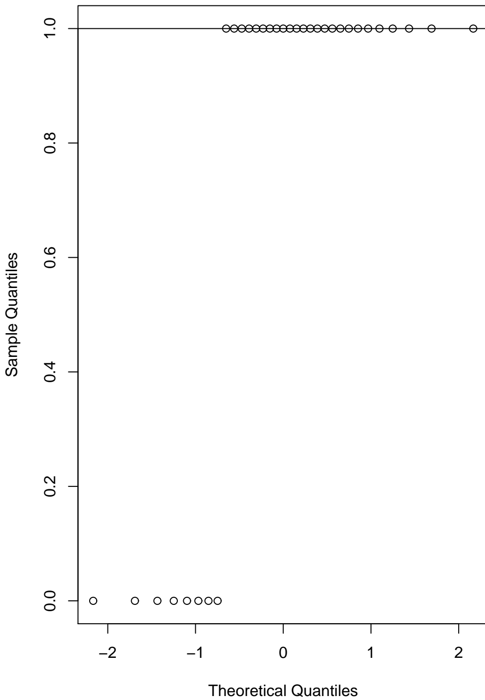
Normal QQplot – Variable 2
