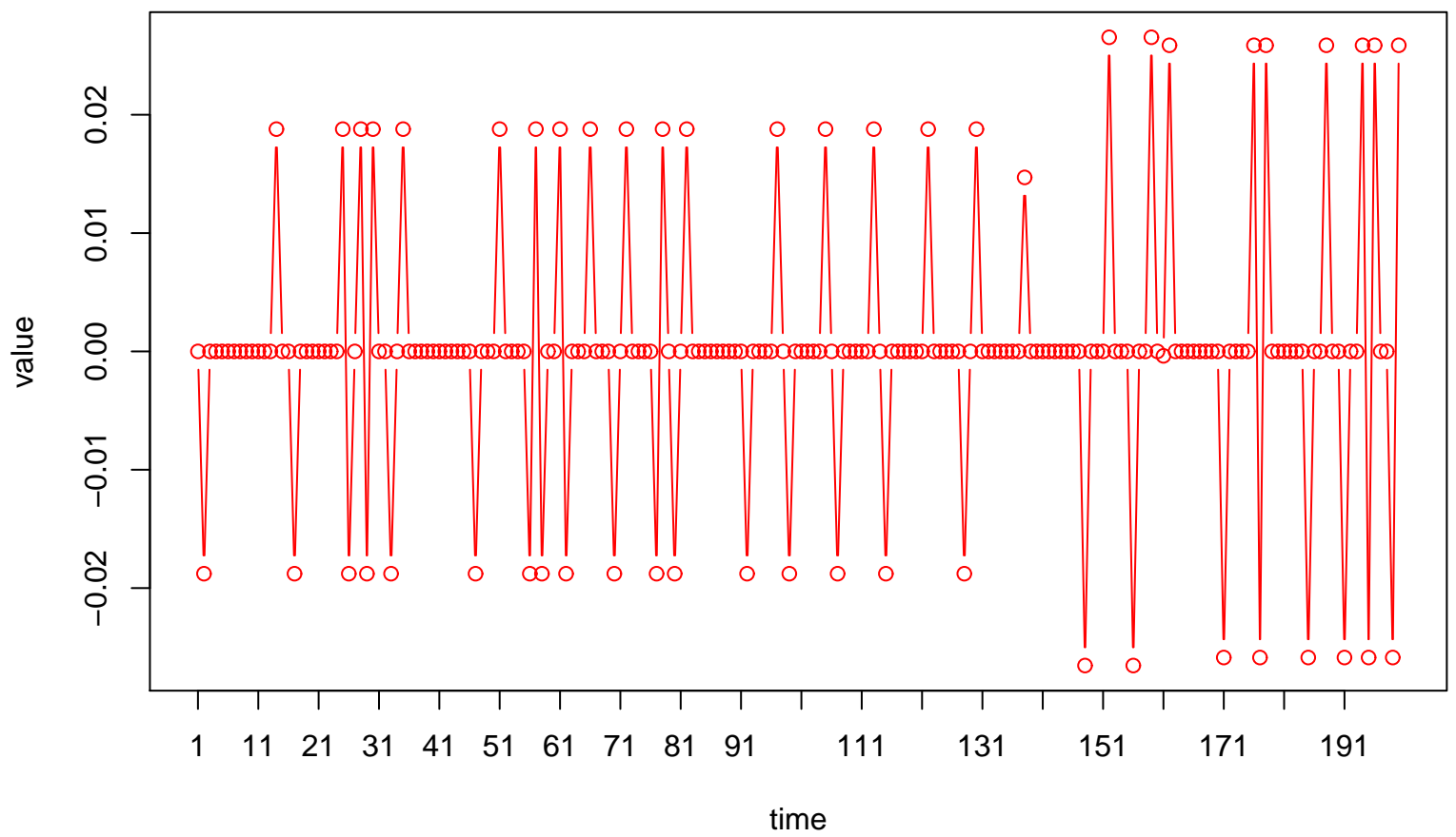
Time Plot of Techcars Log>Returns
