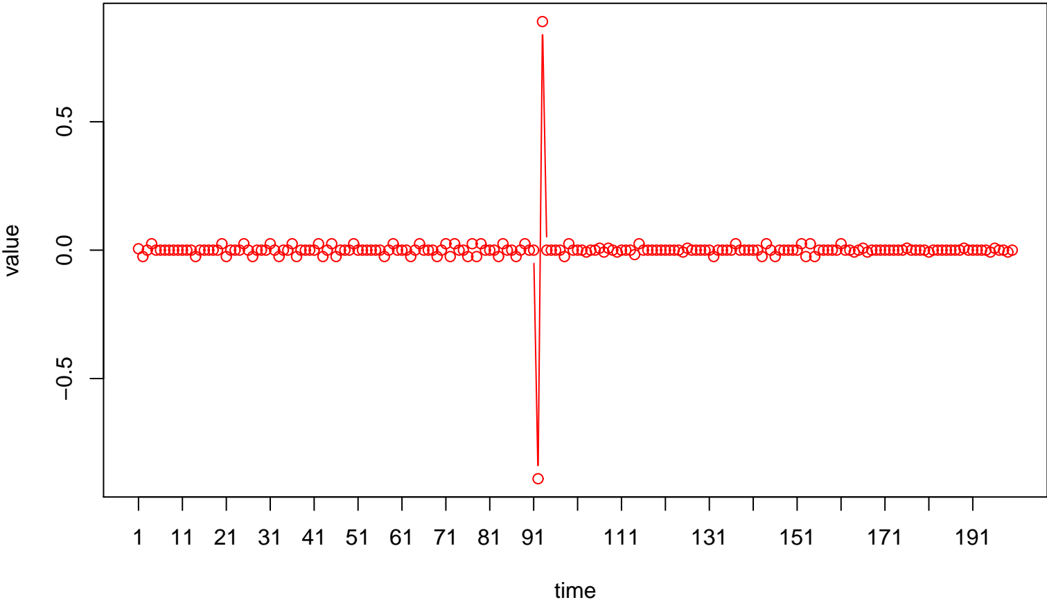
Time Plot of Chemco Log-Returns
