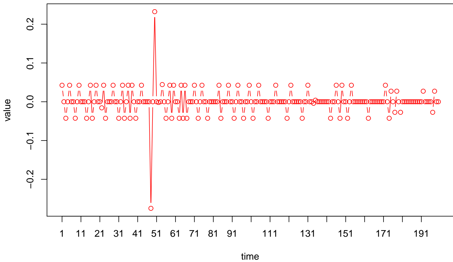
Time Plot of Northern Gunman Log-Returns
