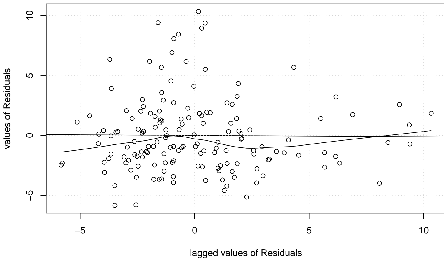
Residual Lag plot, lowess, and regression line
