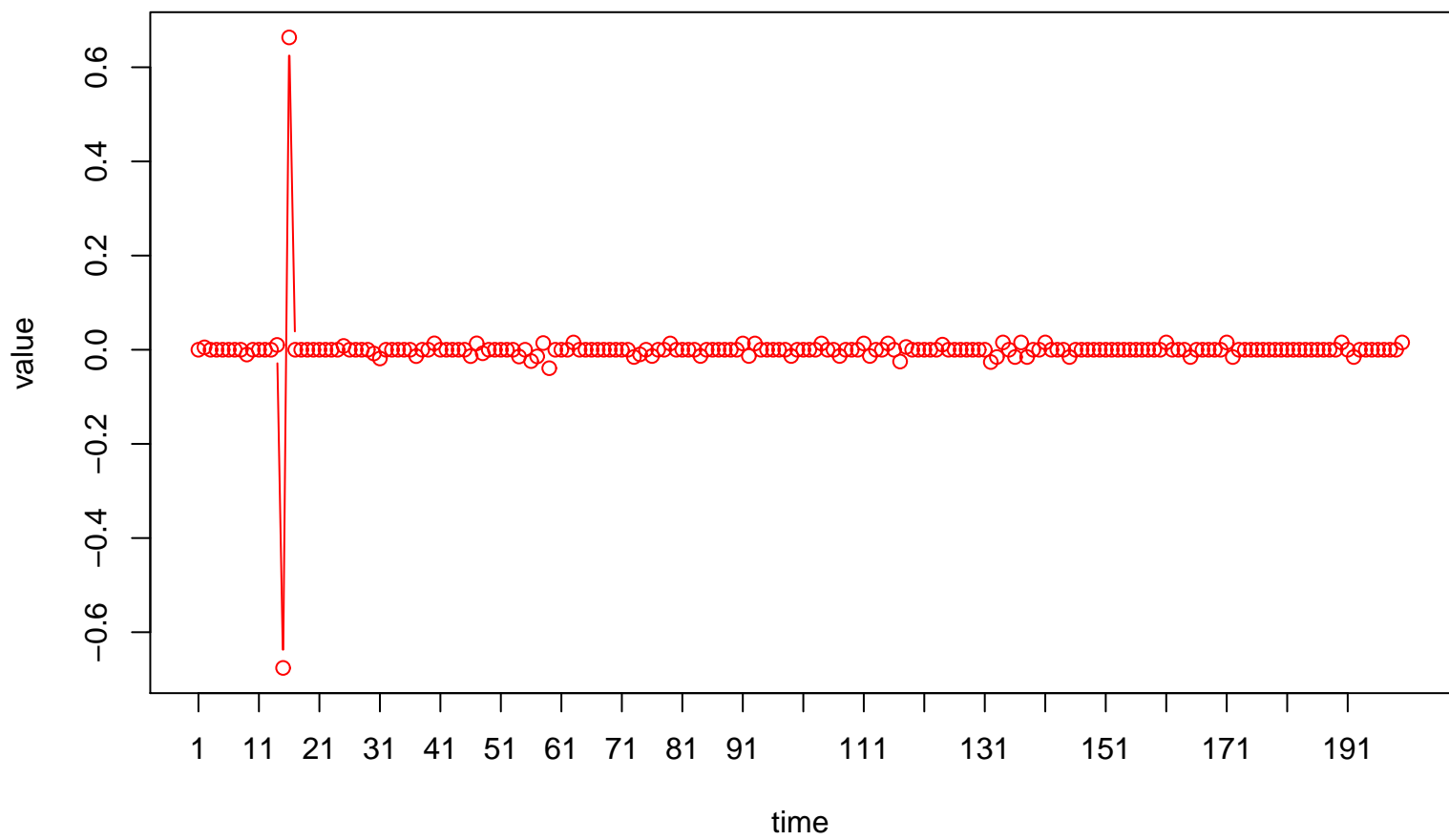
Time Plot of Green & Blue Log-Returns
