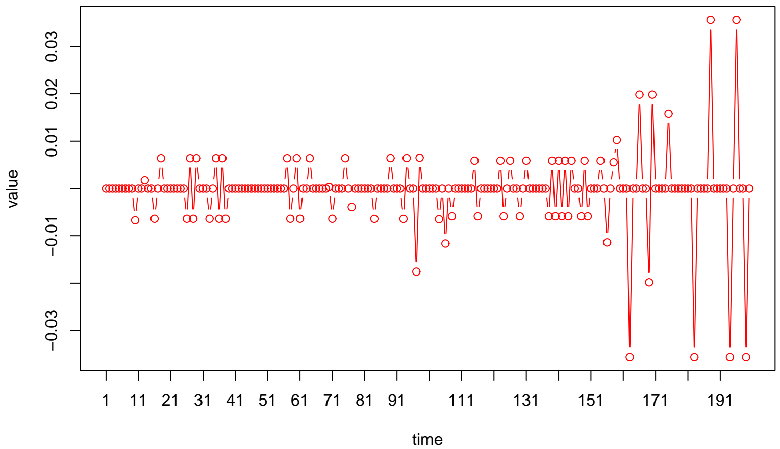
Time Plot of Apollo Oil Corp. Log>Returns
