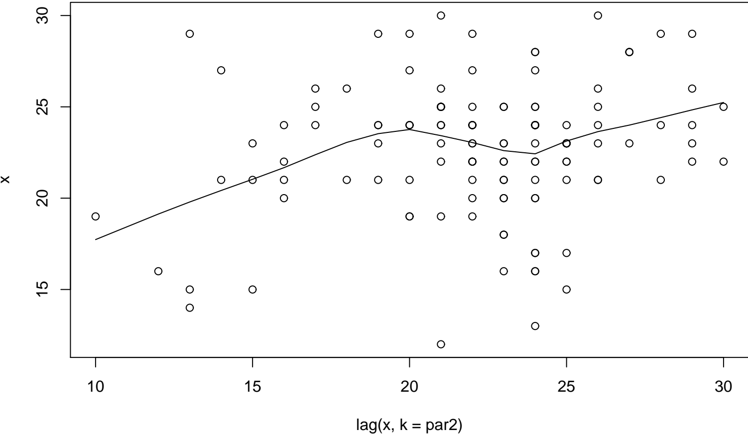
Lag plot (k=32), and lowess
