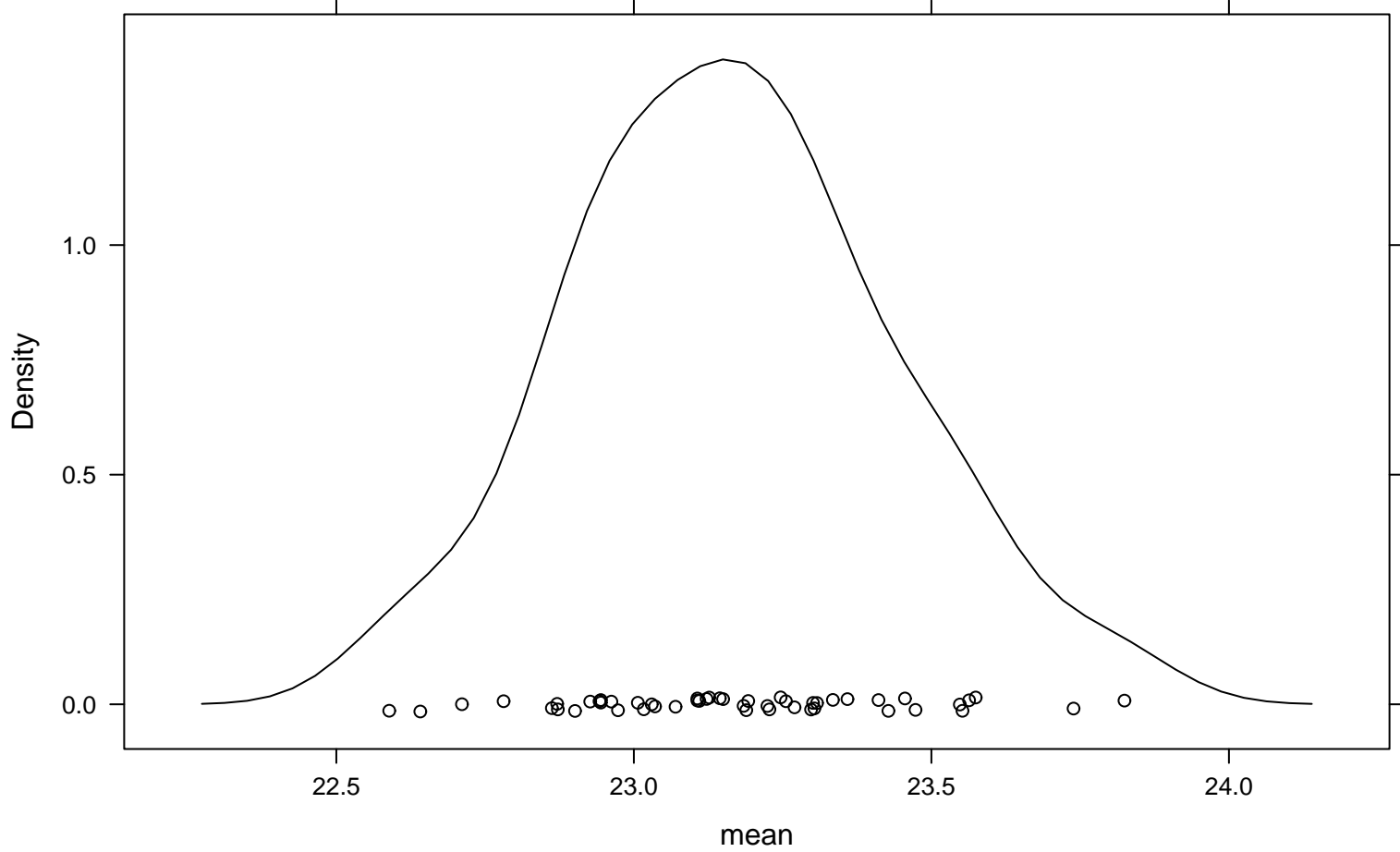
Density Plot
