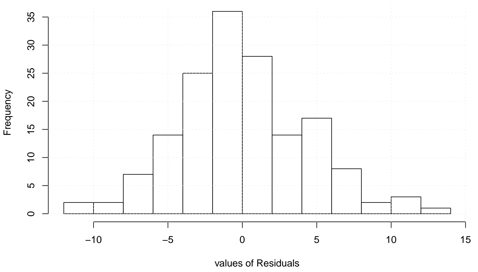
Residual Histogram
