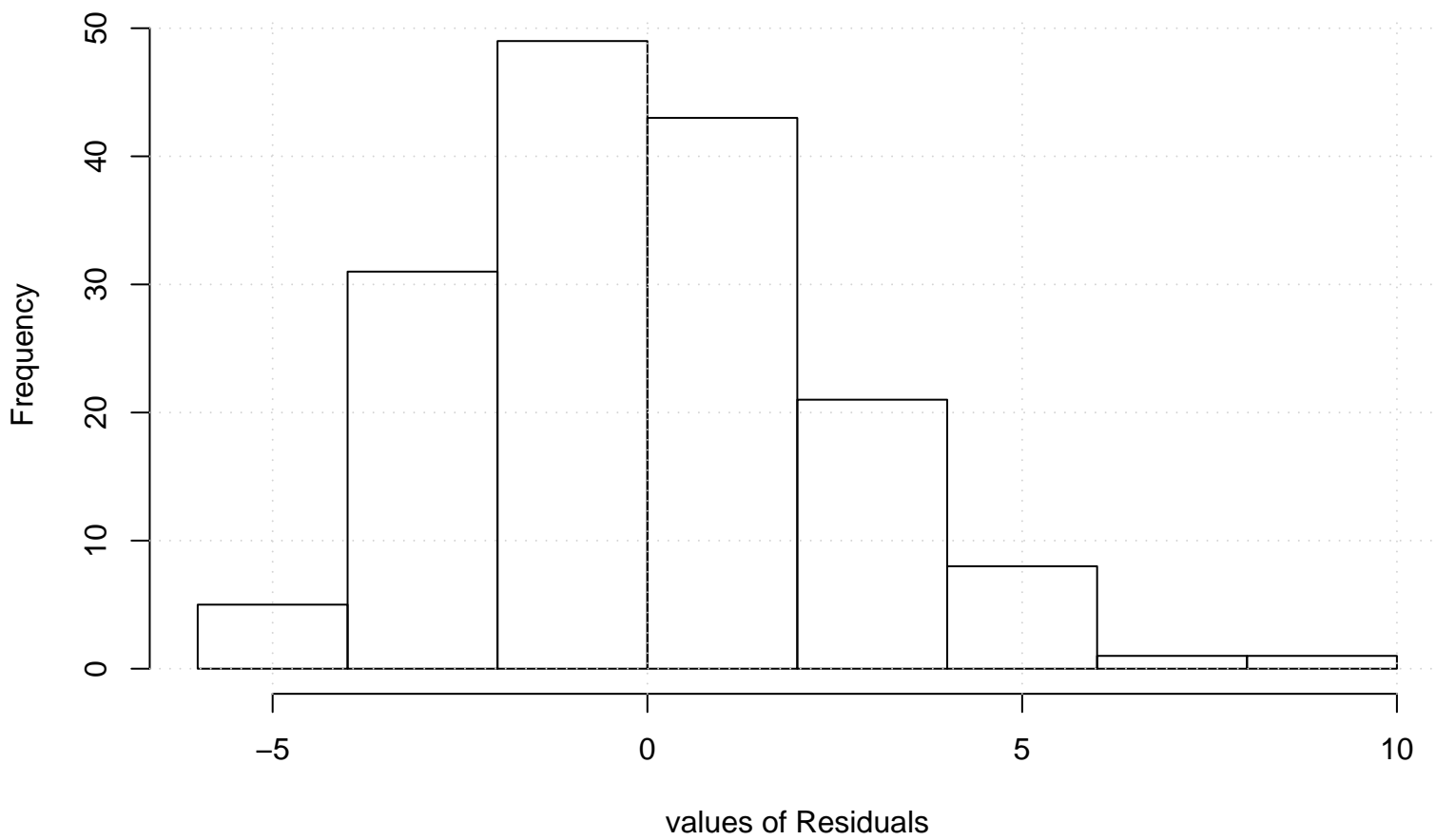
Residual Histogram
