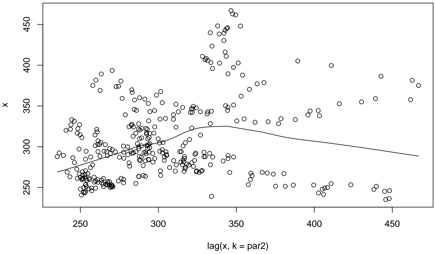
Lag plot (k=20), and lowess
