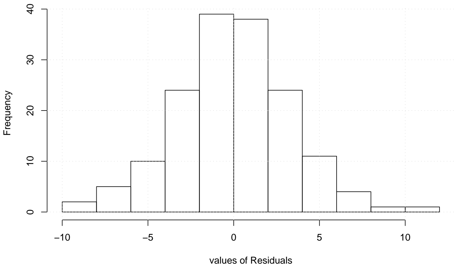
Residual Histogram
