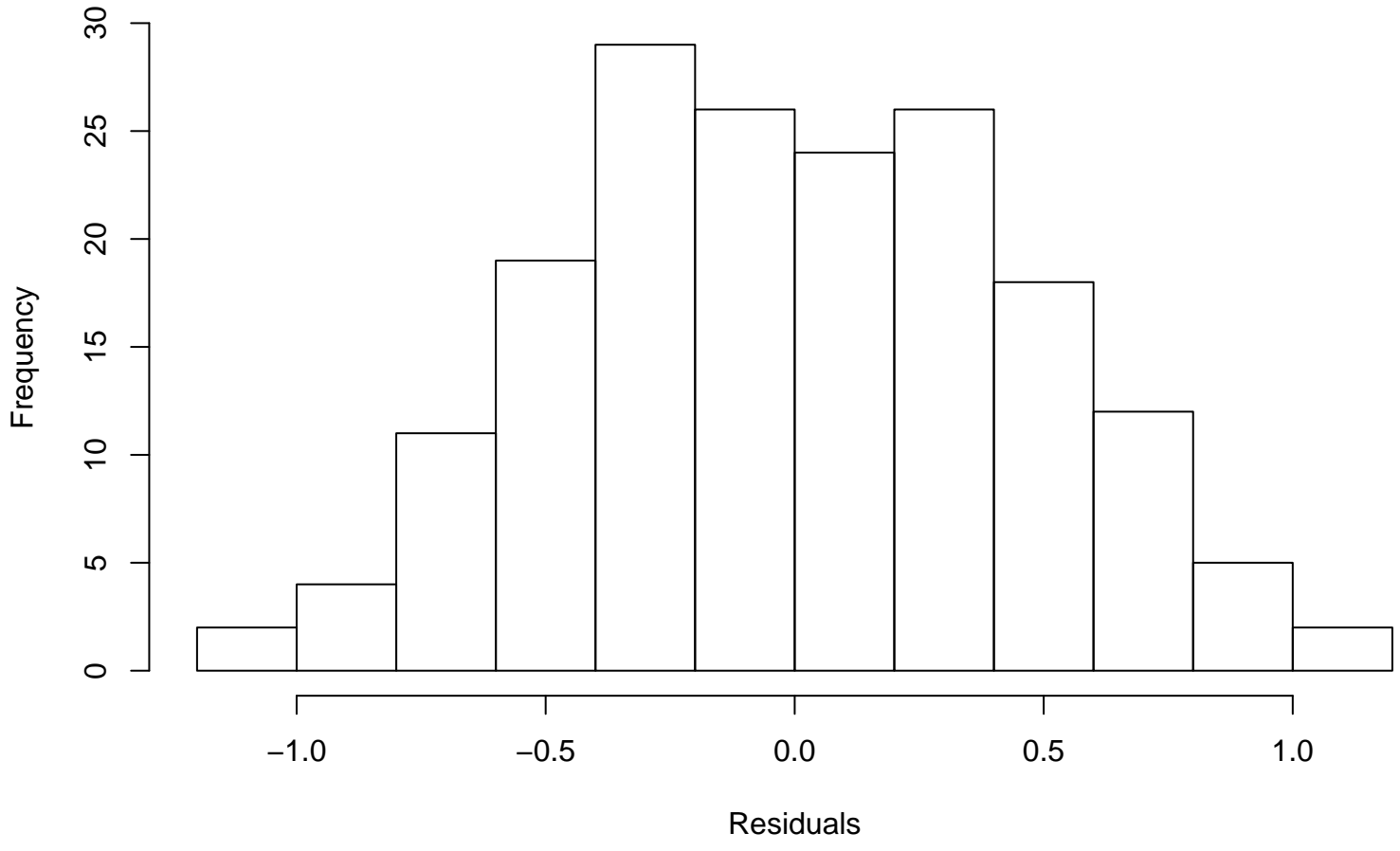
Residual Histogram
