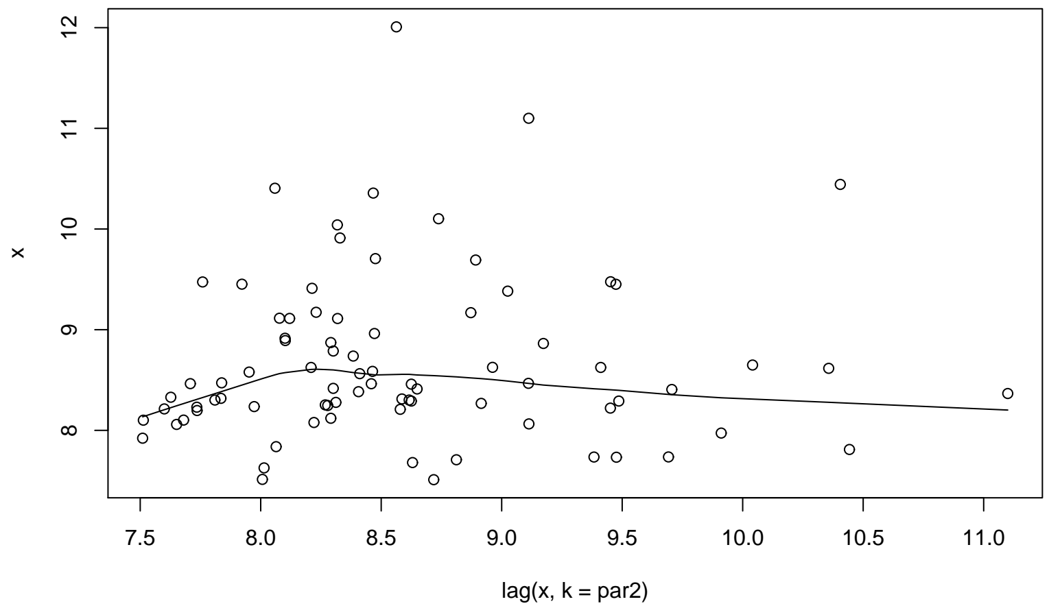
Lag plot (k=15), and lowess
