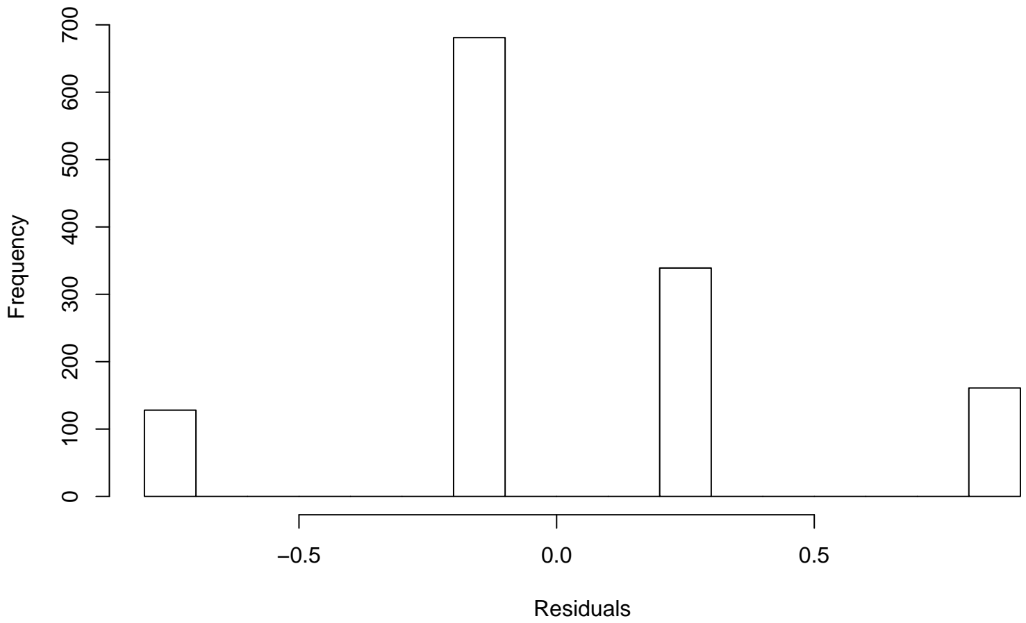
Residual Histogram
