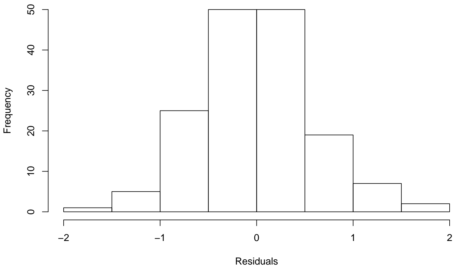
Residual Histogram
