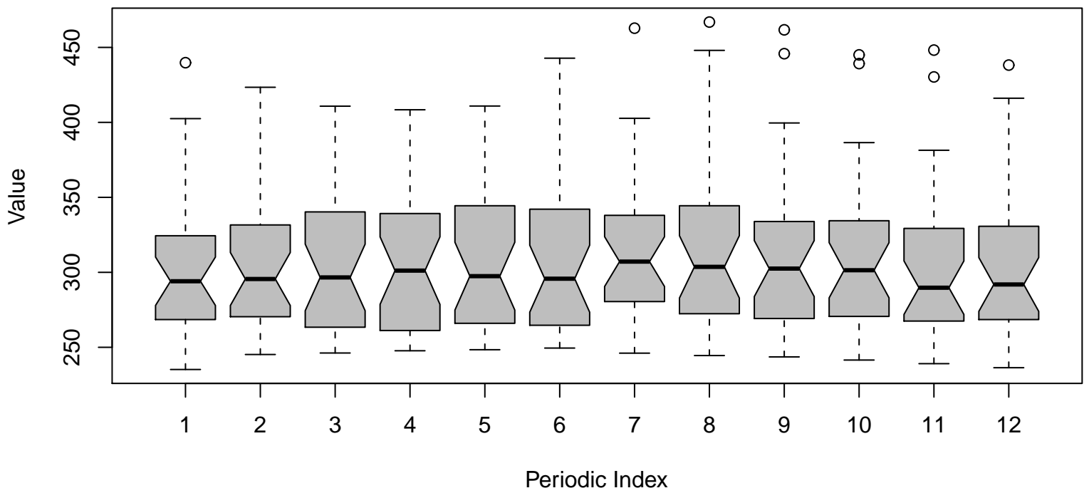
Notched Box Plots – Periodic Subseries
