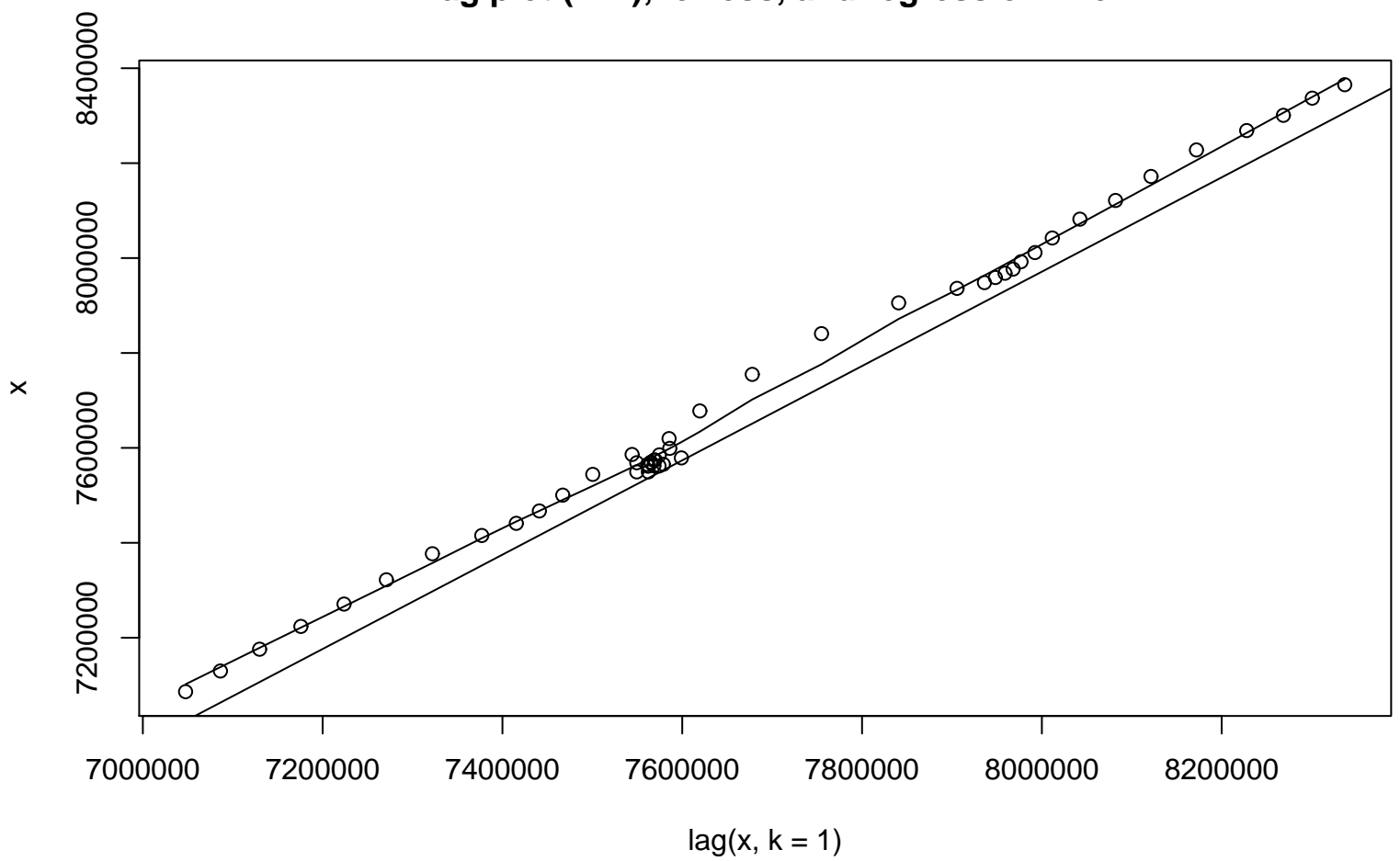
Lag plot (k=1), lowess, and regression line
