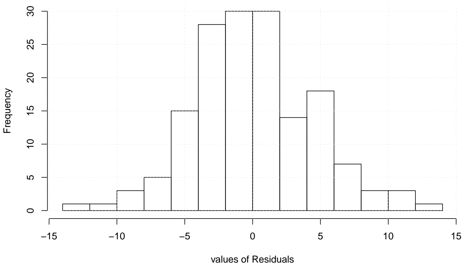
Residual Histogram
