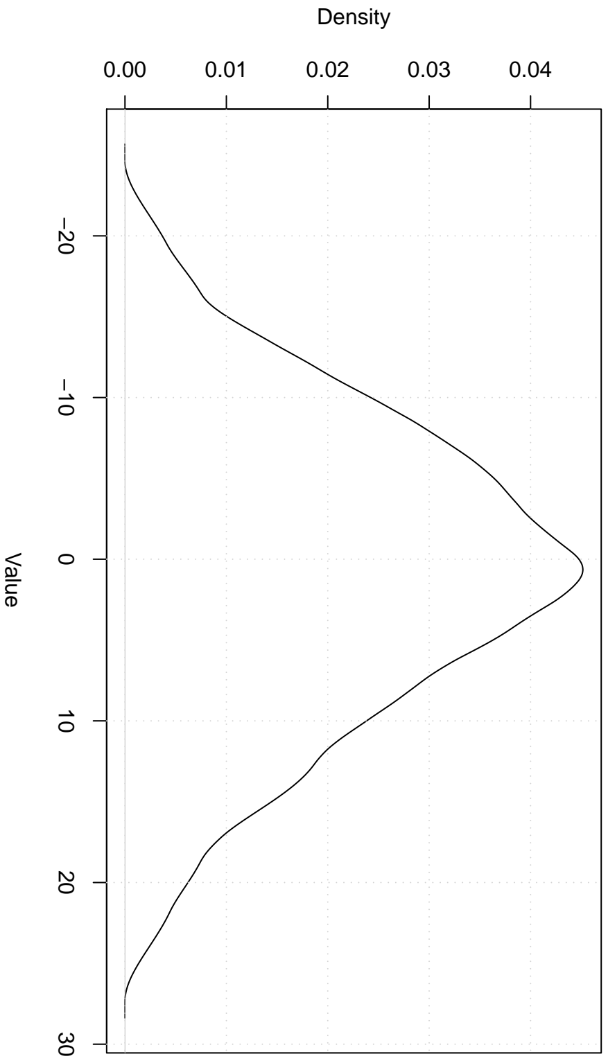
Biweight Kernel
