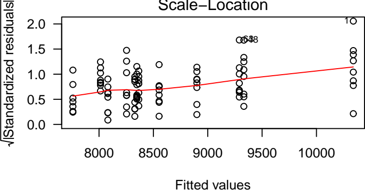
Scale-Location
