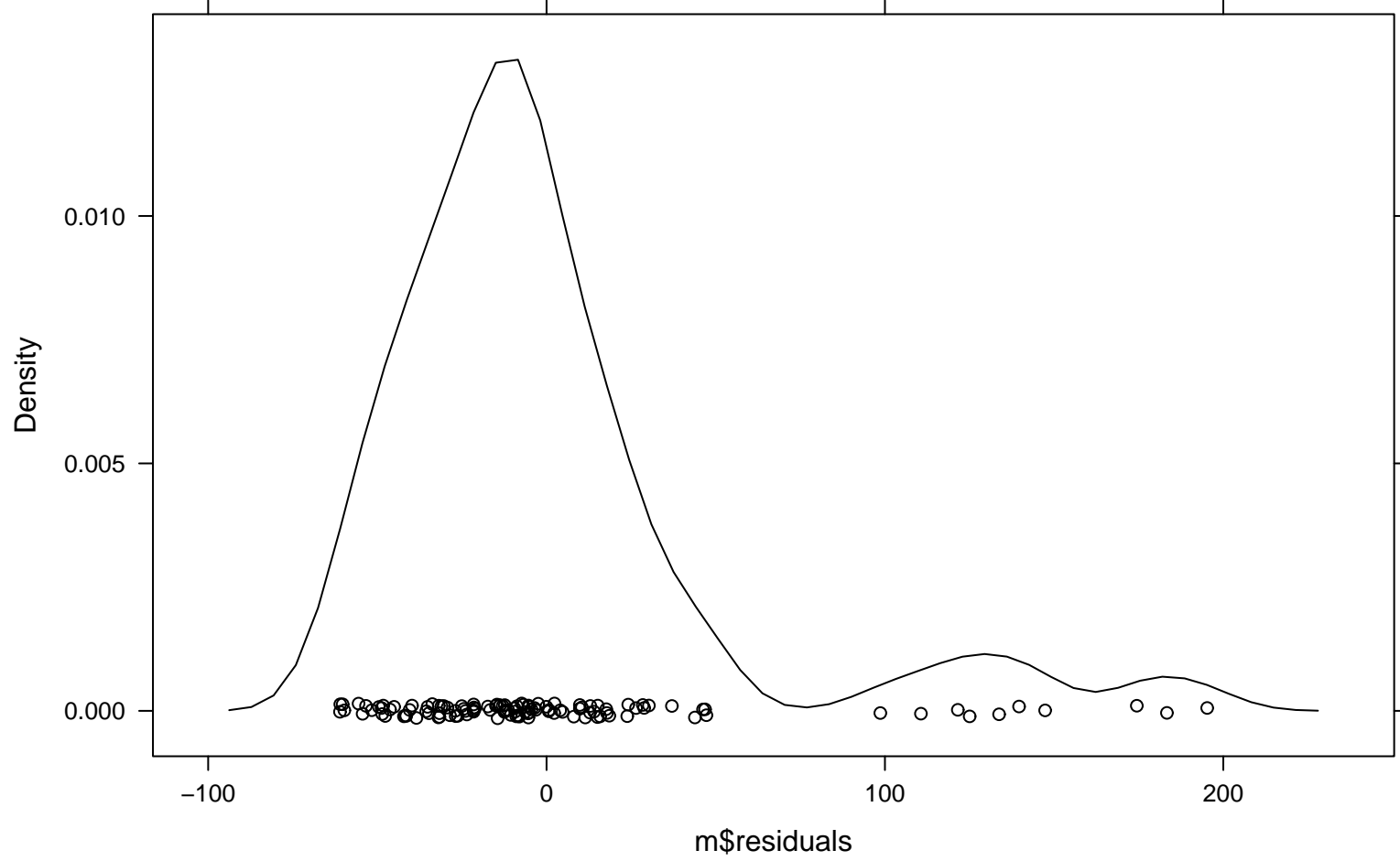
Density Plot
