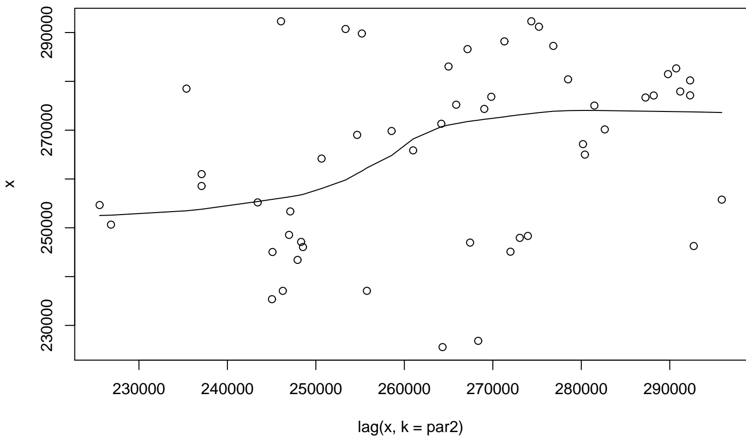
Lag plot (k=8), and lowess
