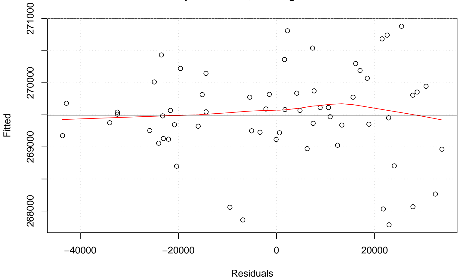
Scatterplot, lowess, and regression line
