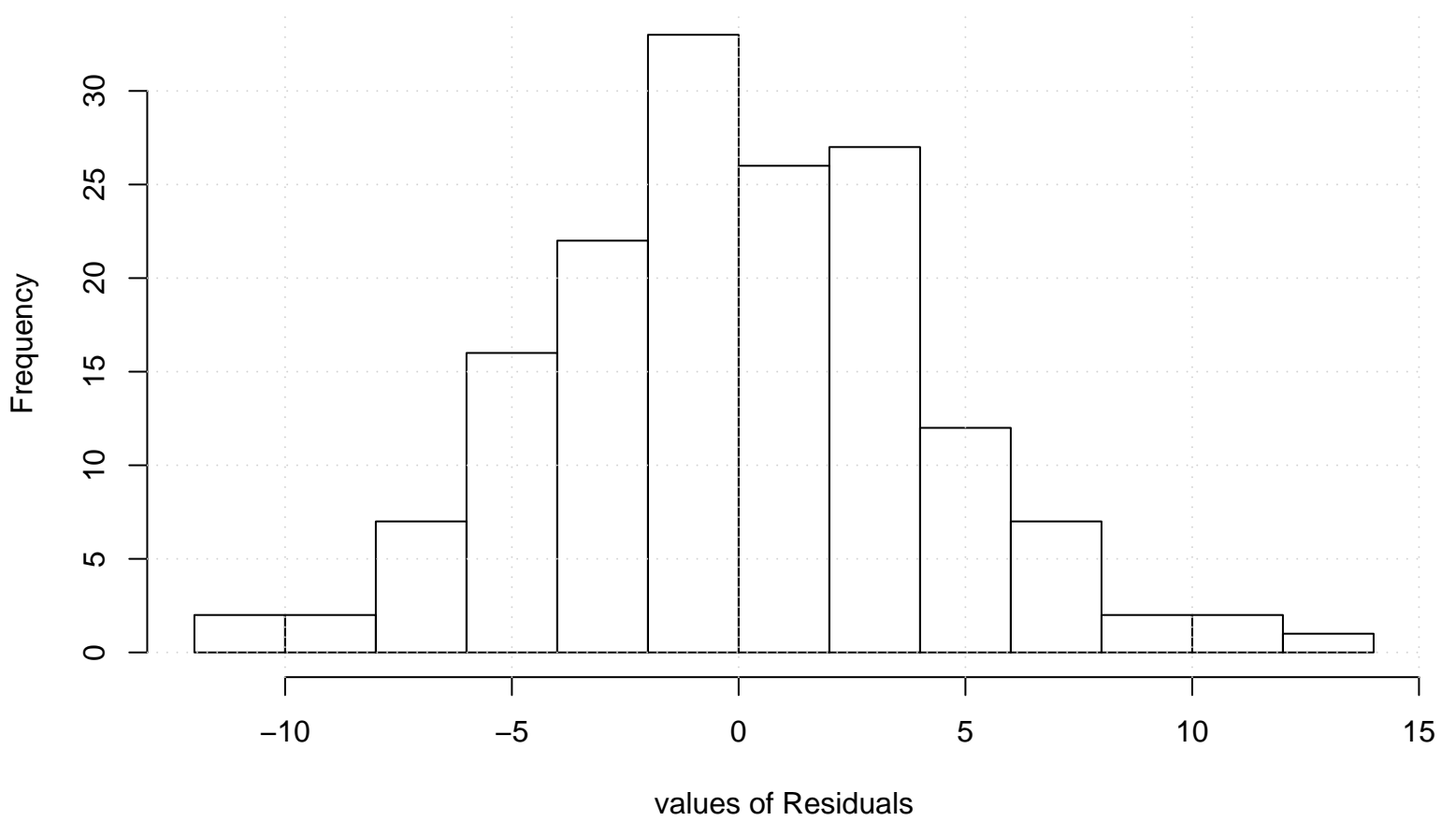
Residual Histogram
