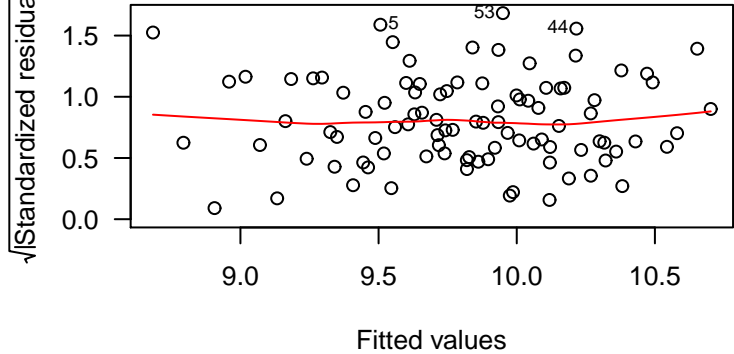
Scale-Location
