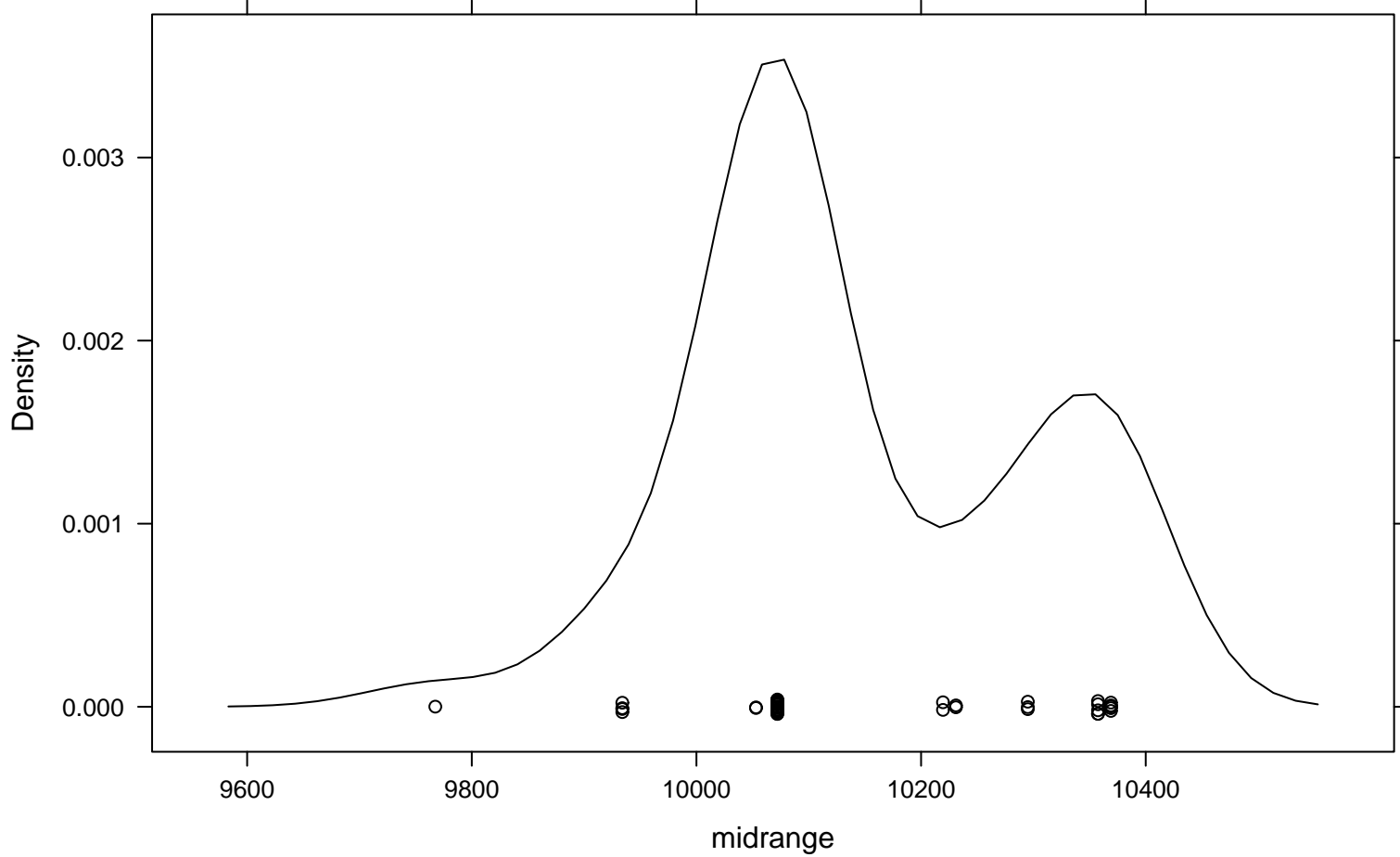
Density Plot
