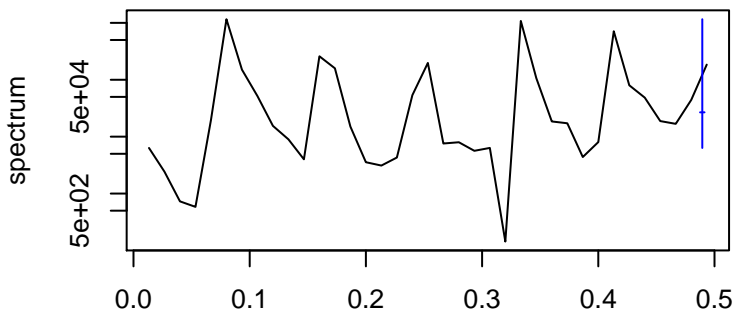
Seasonal
