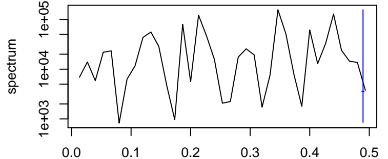
Remainder
