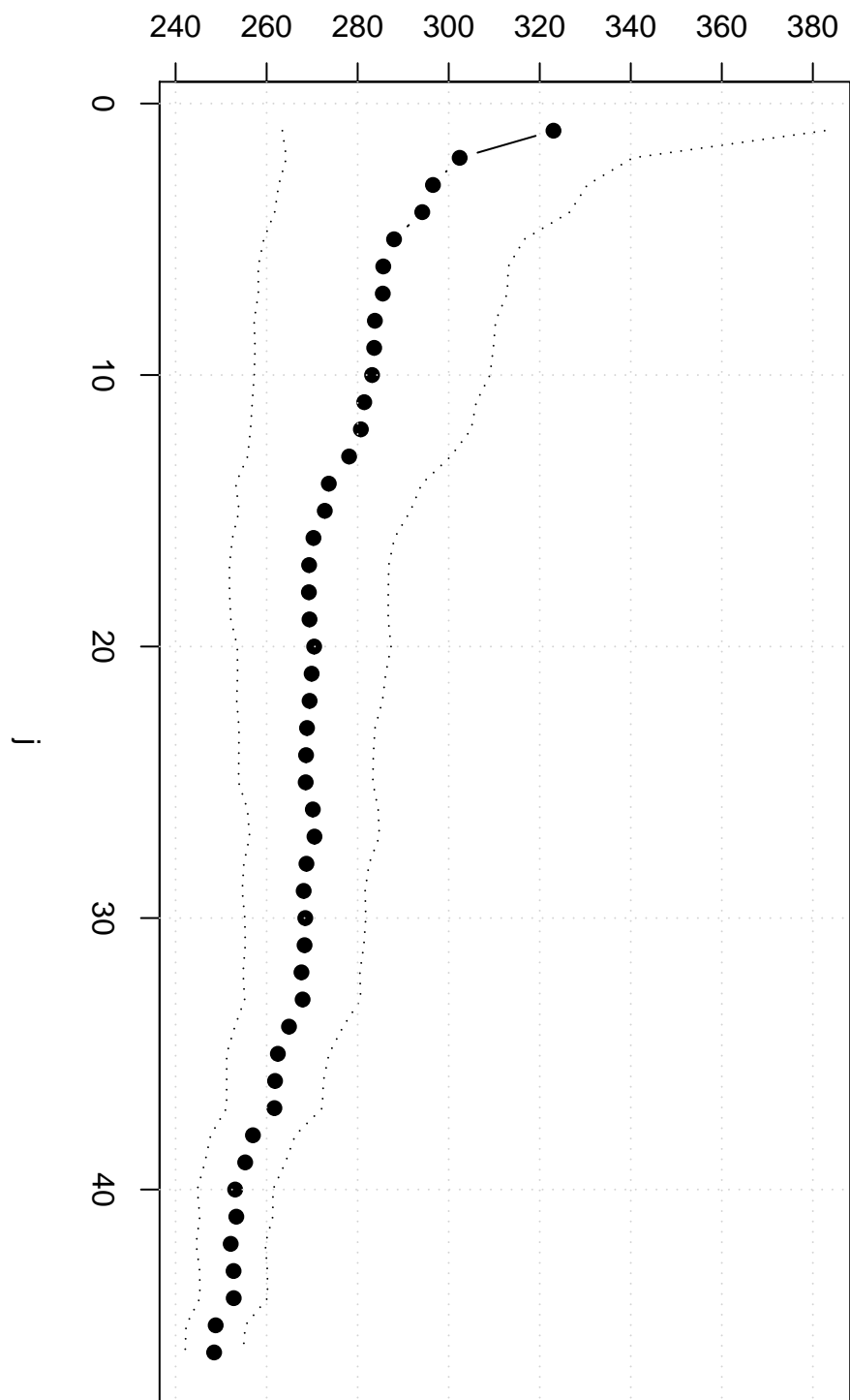
Winsorized Mean(j/n)
