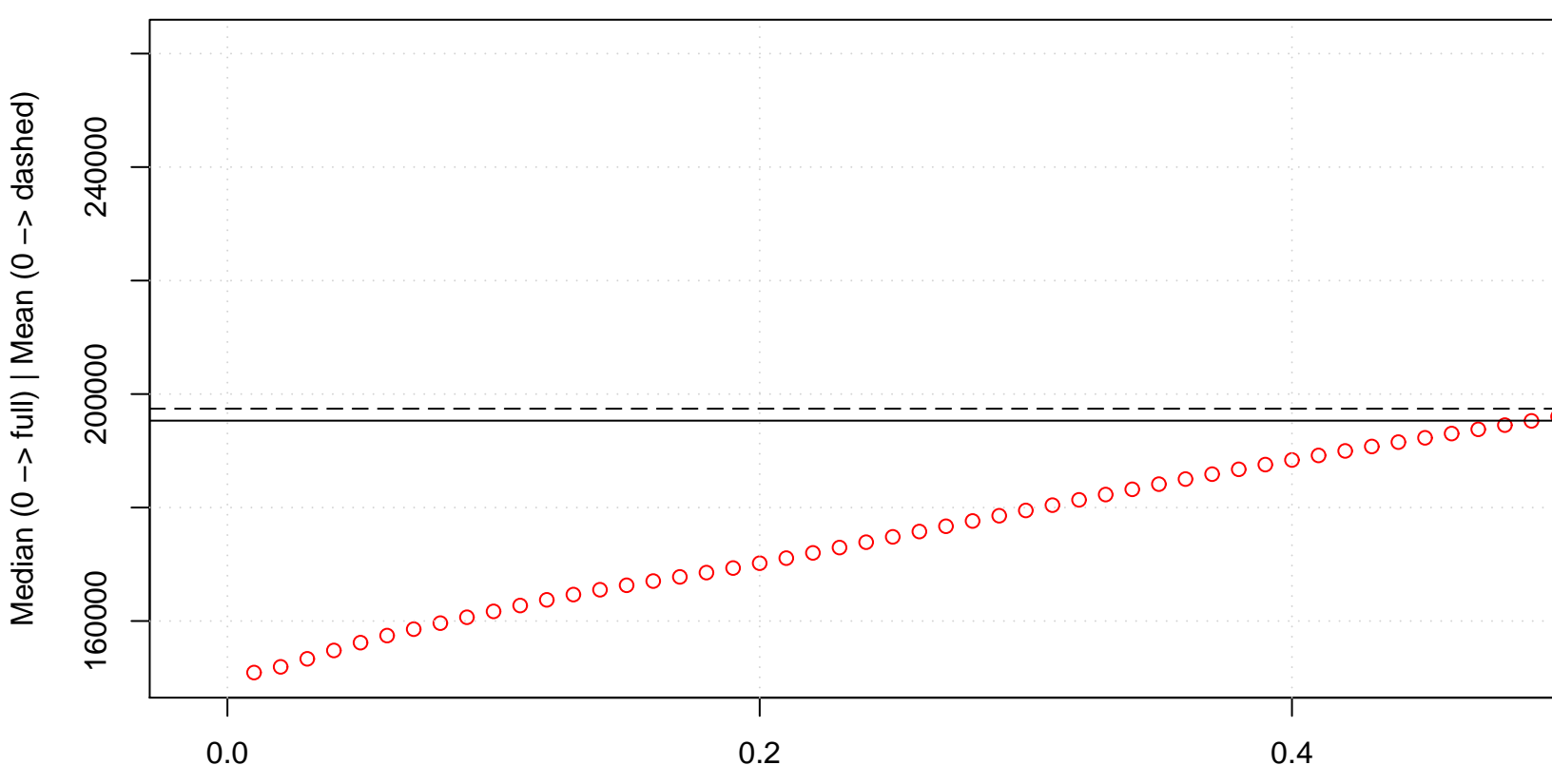
Harrell-Dav
