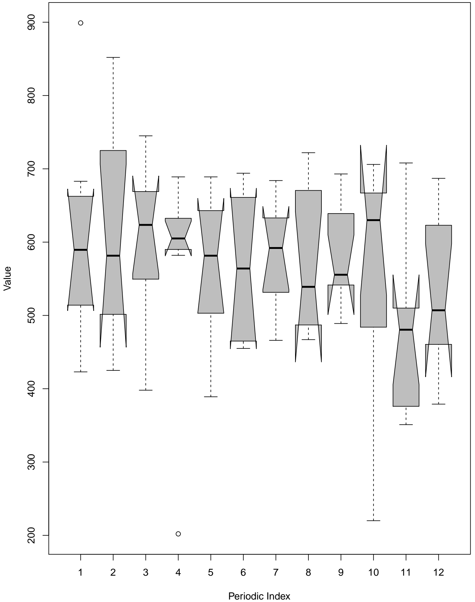
Notched Box Plots – Periodic Subseries
