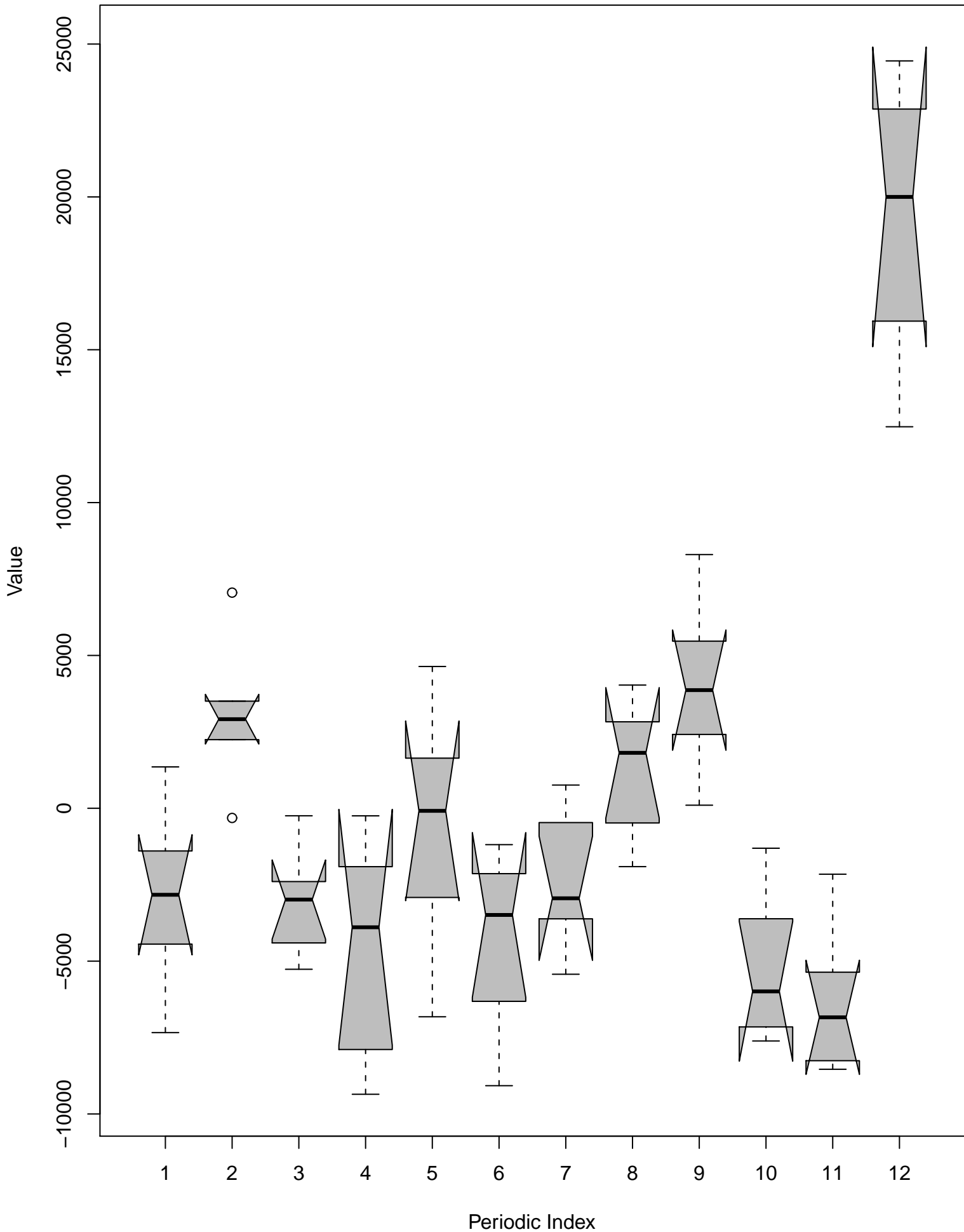
Notched Box Plots – Differenced Periodic Subseries
